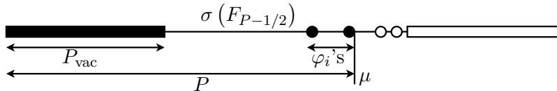
FIG. 3: Decomposition of the system ‘vacuum + N electrons’ for the solution P in the N th charge sector.
